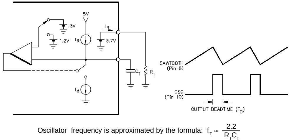
FIGURE 20 - OSCILLATOR CIRCUIT
