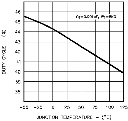
FIGURE 18. DUTY CYCLE VS. TEMPERATURE
