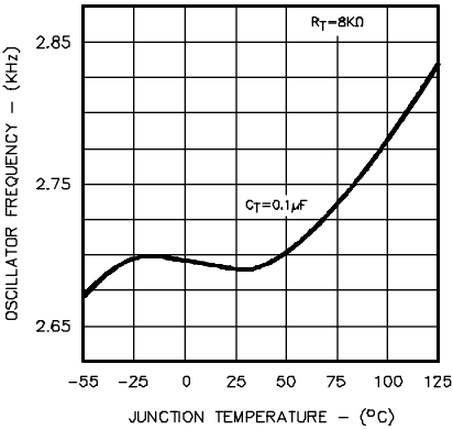
FIGURE 17. OSCILLATOR FREQUENCY VS. TEMPERATURE
