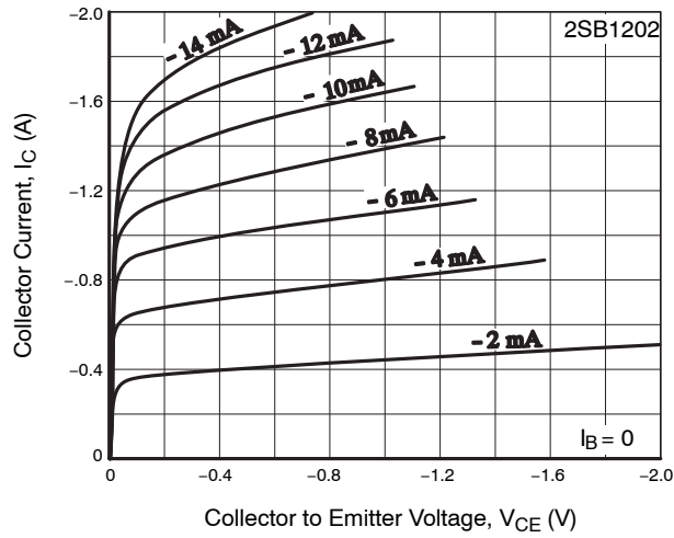
Figure 3. I_C - V_{CE}
