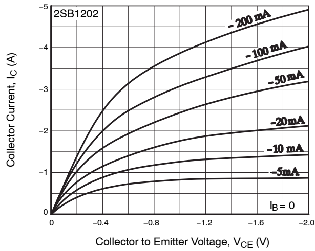
Figure 1. I_C - V_{CE}
