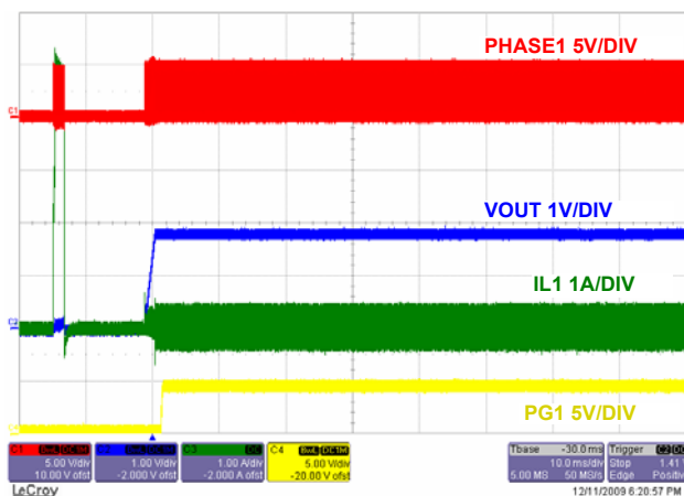
FIGURE 63. OUTPUT SHORT CIRCUIT RECOVERY (FROM HICUP) CHANNEL 1
