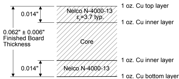
PCB 1093782 Material and Stack-Up
