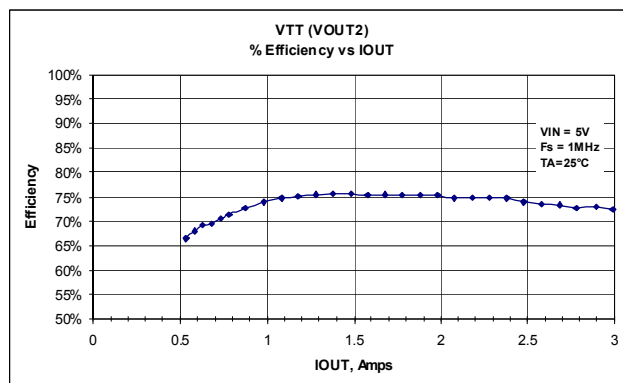
Figure 5. % Efficiency vs. I_{\text{OUT}}
