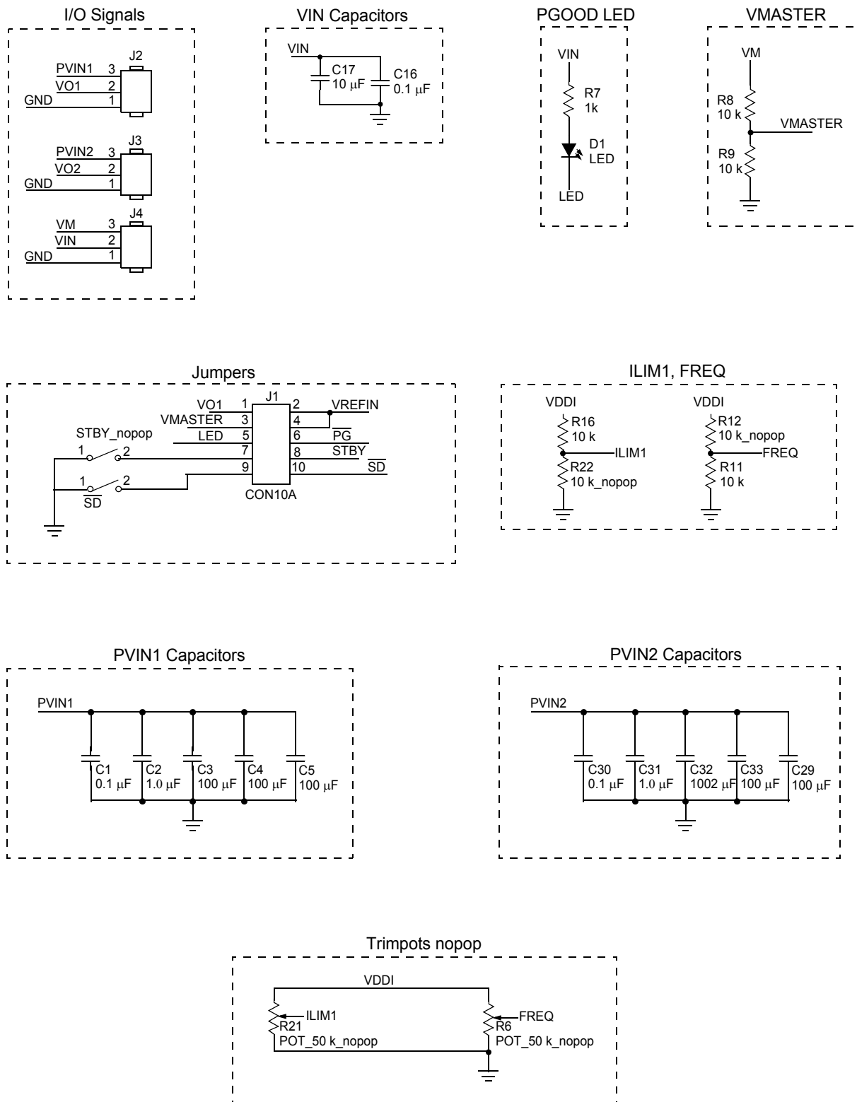
Figure 10. 34716 Typical Application
