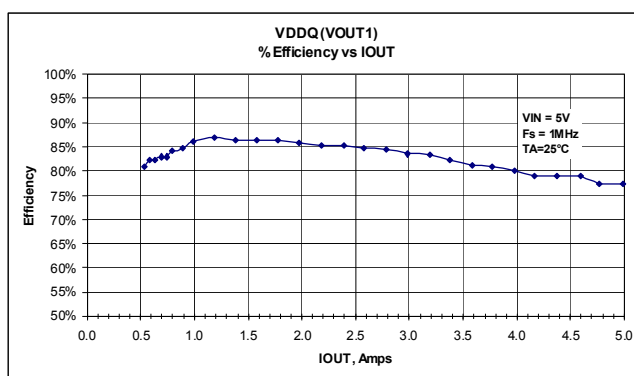
Figure 4. % Efficiency vs. I_{\text{OUT}}
