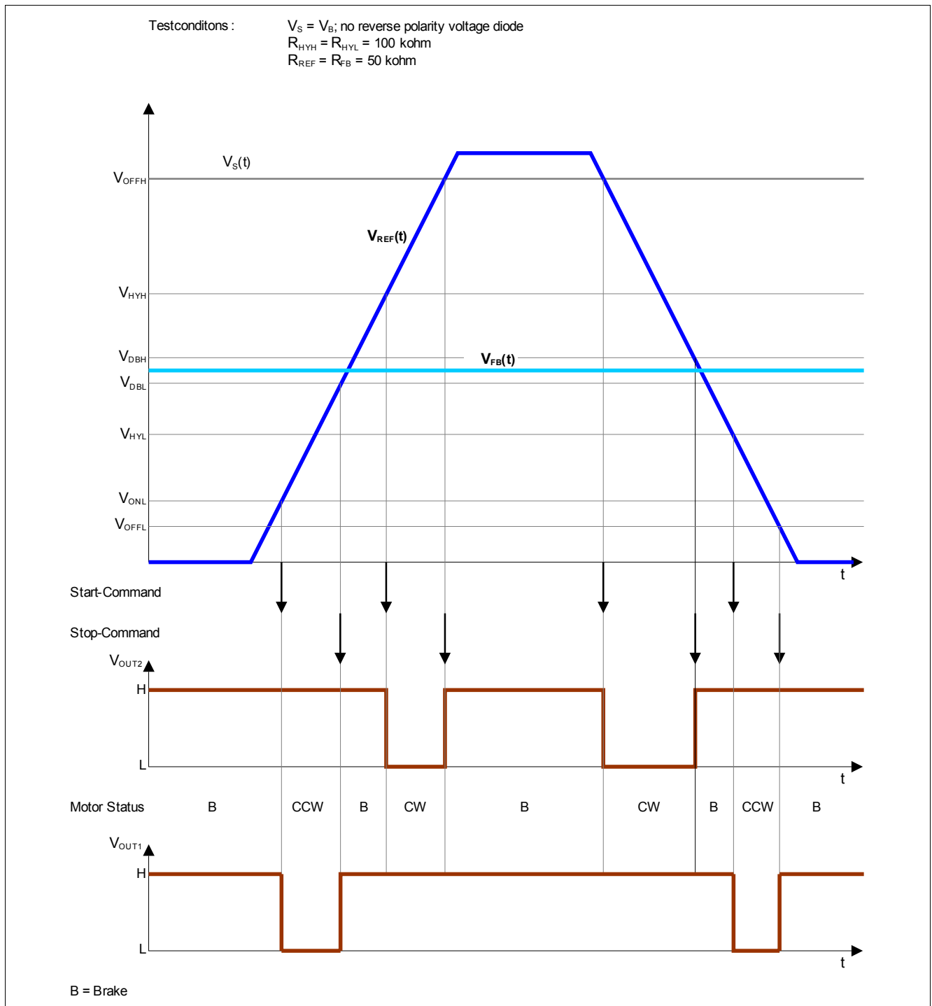
Figure 5 Motor Operation
