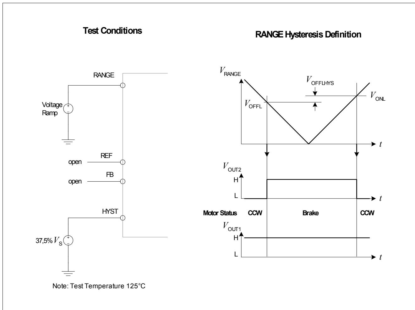
Figure 6 RANGE Hysteresis and Test Conditions
