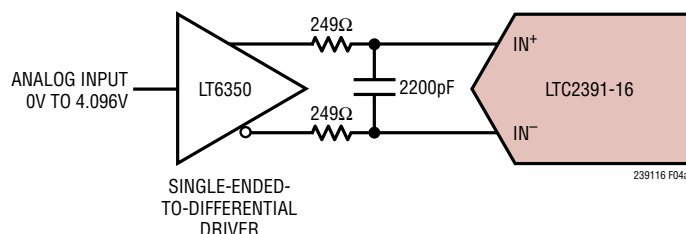
Figure 4a. Recommended Single-Ended-to-Differential Conversion Circuit Using the LT6350 ADC Driver
