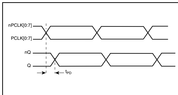
Propagation Delay
