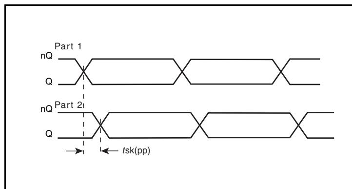
Part-to-Part Skew
