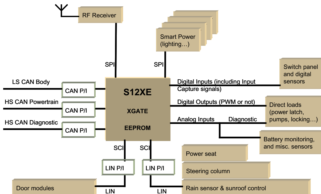
Figure 1. Body Controller Application Example
