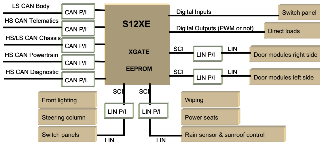
Figure 2. Gateway Application Example
