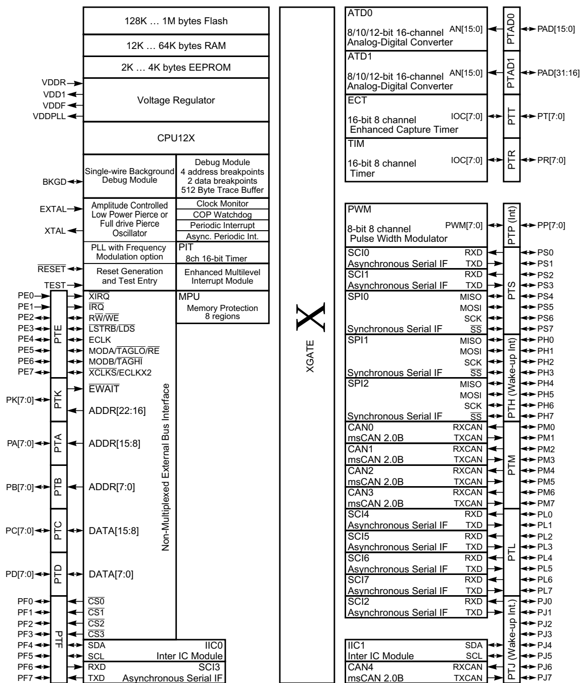
Figure 3. MC9S12XE Block Diagram
