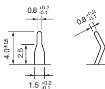
(Terminal dimensions)
