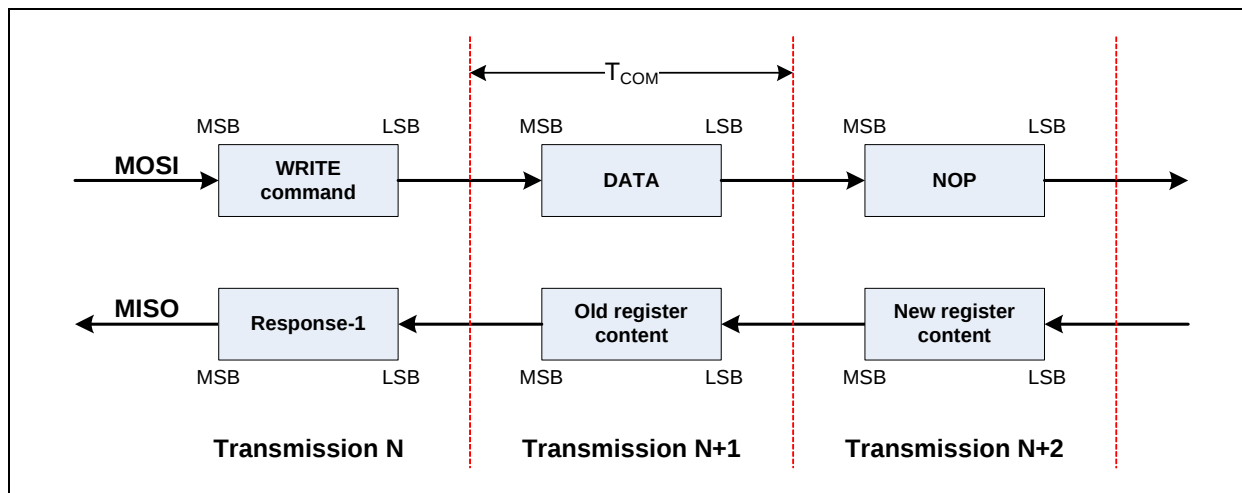
Figure 24: WRITE Command
