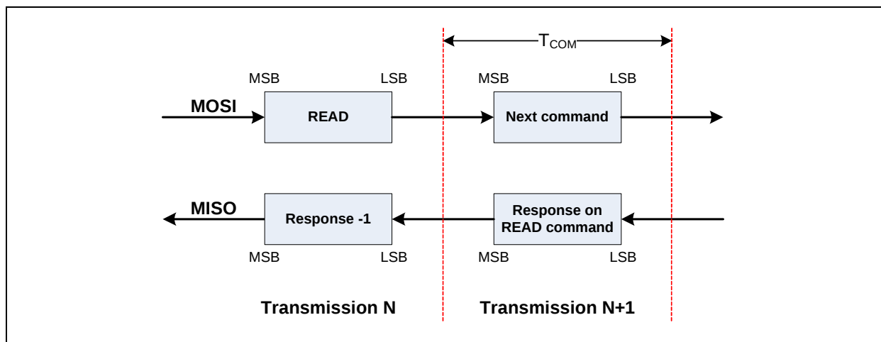
Figure 23: READ Command
