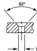
GT02RFS Countersunk holes required when mating with GT06CFGG, page 55 and GT08CFGG, page 73
