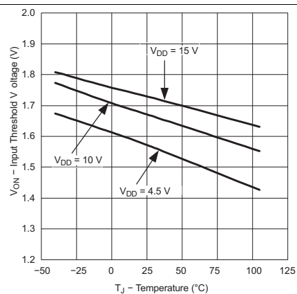
Figure 23. Input Threshold vs Temperature
