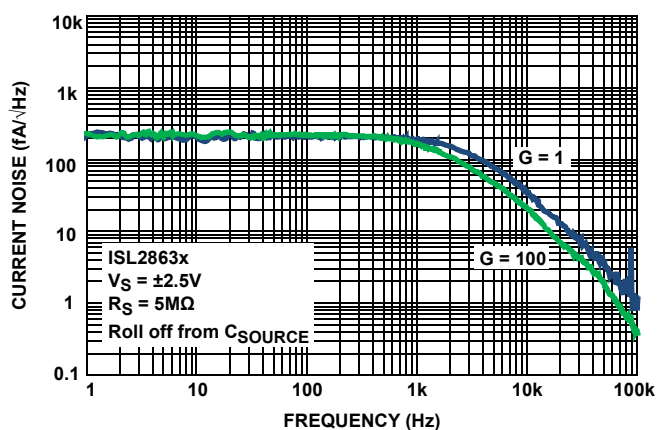
FIGURE 36. PGIA CURRENT NOISE SPECTRAL DENSITY 1Hz TO 100kHz, ISL2863x
