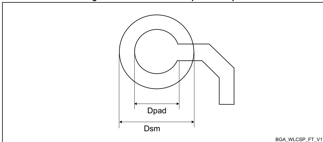
Figure 72. UFBGA100 - Footprint example
