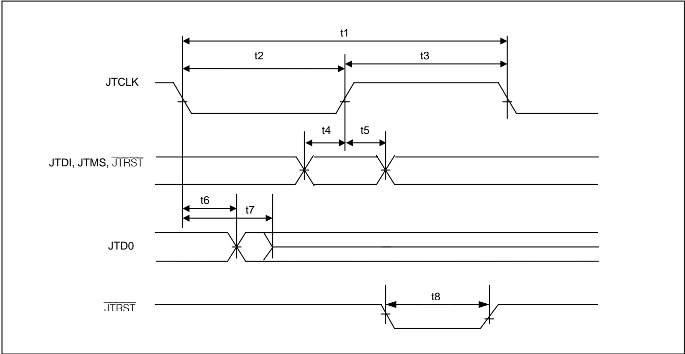
Figure 13-13. JTAG Interface Timing Diagram
