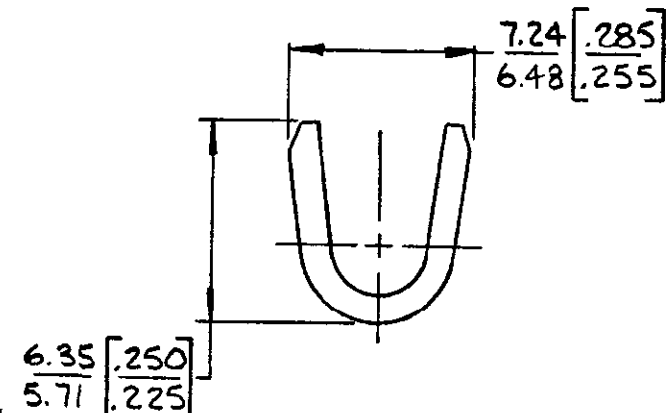
SECT B-B
