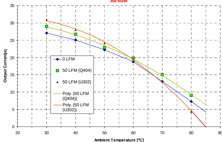
QHS35-033 Thermal Derating
