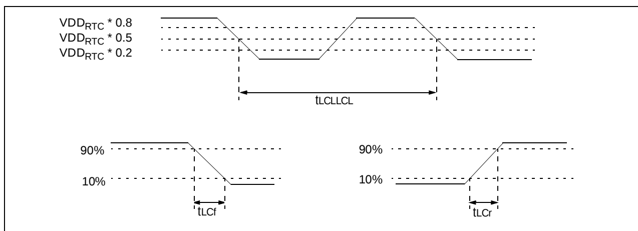
Figure 17: CLKIN timings
