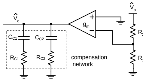
Figure 31. Compensation Network
