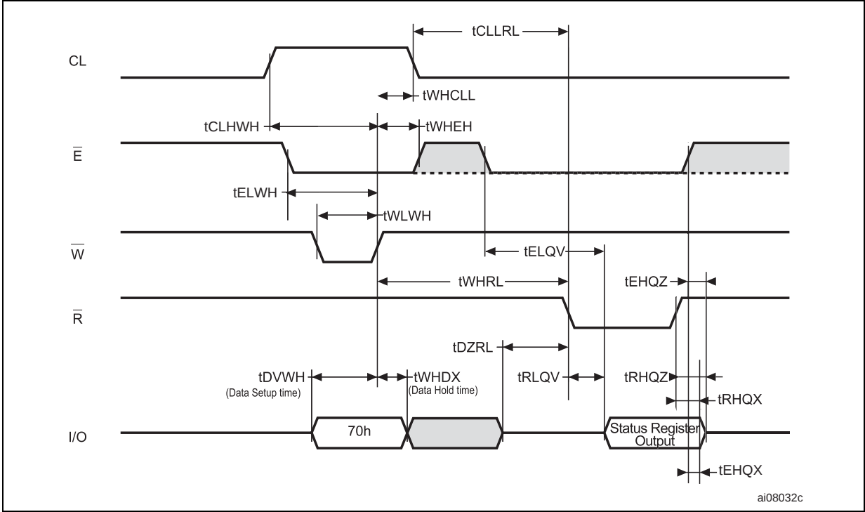
Figure 22. Read status register AC waveforms
