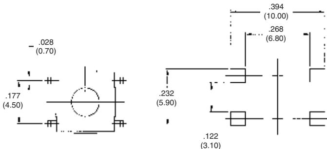
PCB Land Dimension
