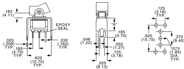
Vertical Support Bracket Single Pole
