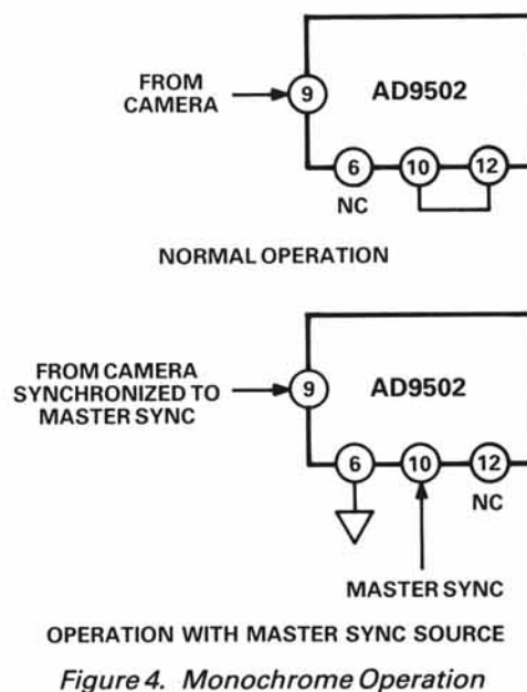
Figure 4. Monochrome Operation
