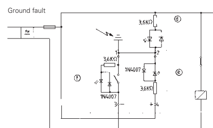
Earth Disconnect terminal with Neon Lamp
