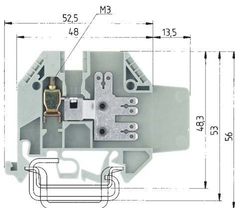
Push-on connectors 2.8 x 0.8 accord. to DIN 46247 Push-on connectors 6.3 x 0.8 accord. to DIN 46247
