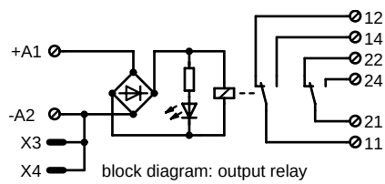
WRS-REL-2W 250 V 5 A
