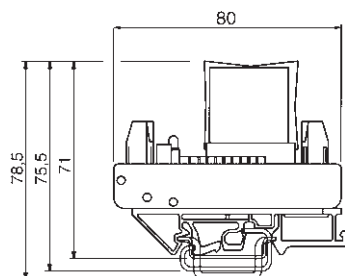
WR4/WR8 – 1 Changeover contact (SPDT)
