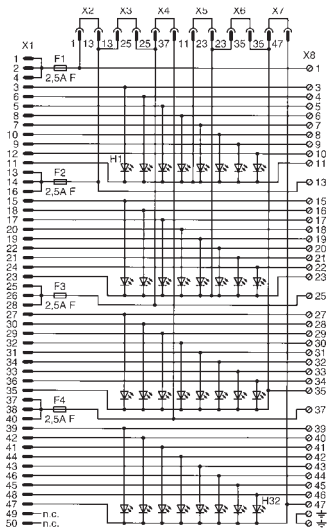
Wiring diagram
