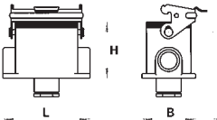
Closed bottom housing with one narrow-side entry cable gland on the left
