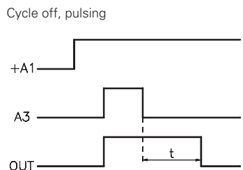
off delay
