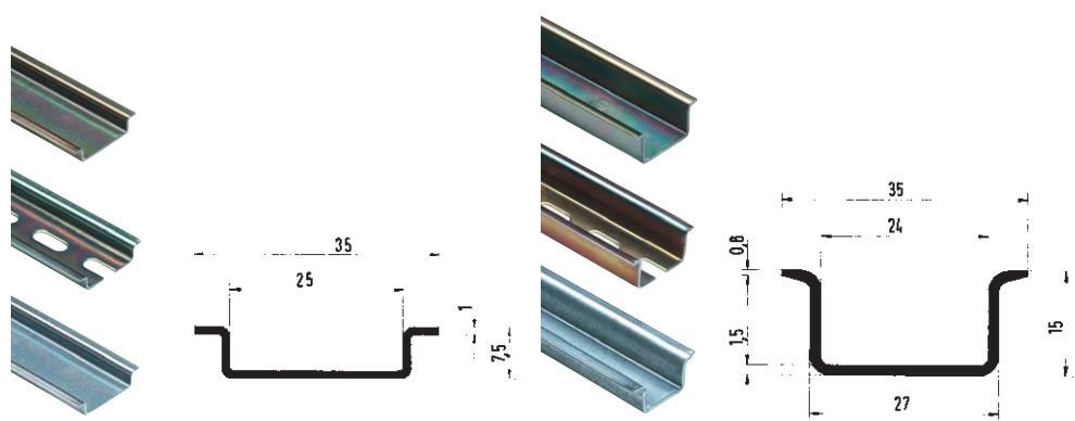
Mounting rail 35 x 7,5 according to DIN EN 60715
