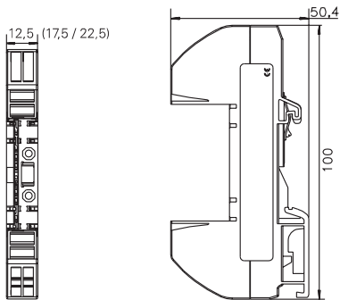
Module board
