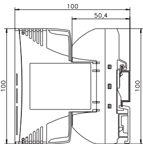
Housing
