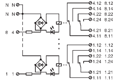
WR4/8-230-2W 250 V 4 A
