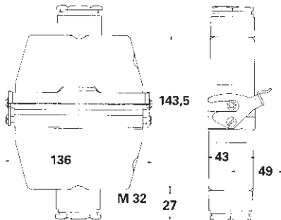
24pole connection
