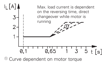
Reversing contactor in dynamic mode
