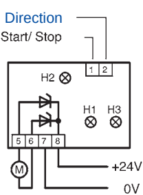
DC motor-reversing contactor
