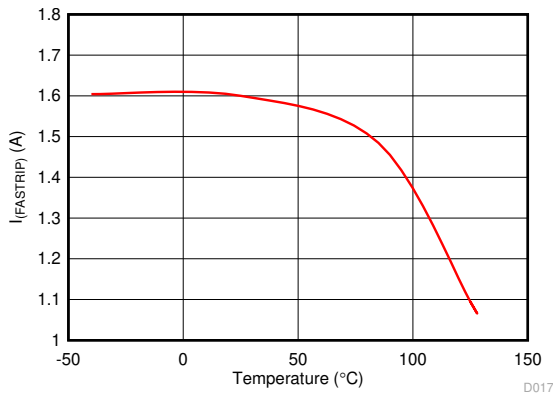
Figure 7-19. Fast-Trip Comparator Threshold I_{\text{FAST-TRIP}} vs Temperature Threshold
