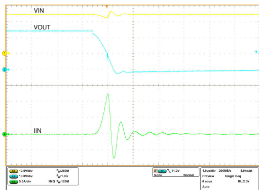
Figure 7-27. Hot-Short: Fast-Trip Response (Zoomed)
