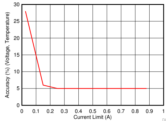
Figure 7-20. Current Limit Accuracy vs Current Limit, I_{\text{OL}}
