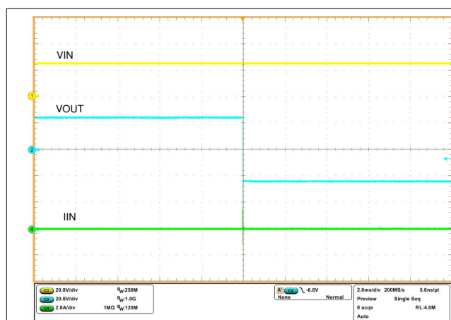
Figure 9-6. Reverse Output Polarity Protection With -24 V at OUT and 24 V at IN
