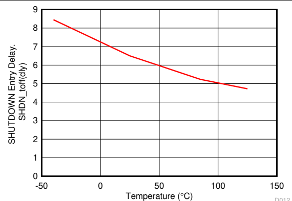
Figure 7-12. Shutdown Entry Delay vs Temperature
