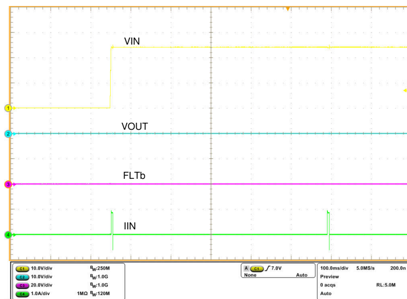
Figure 9-12. Start-Up With Short on Output
