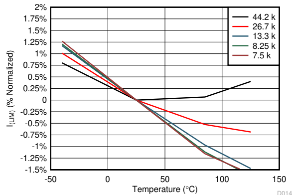
Figure 7-15. Current Limit (% Normalized) vs Temperature
