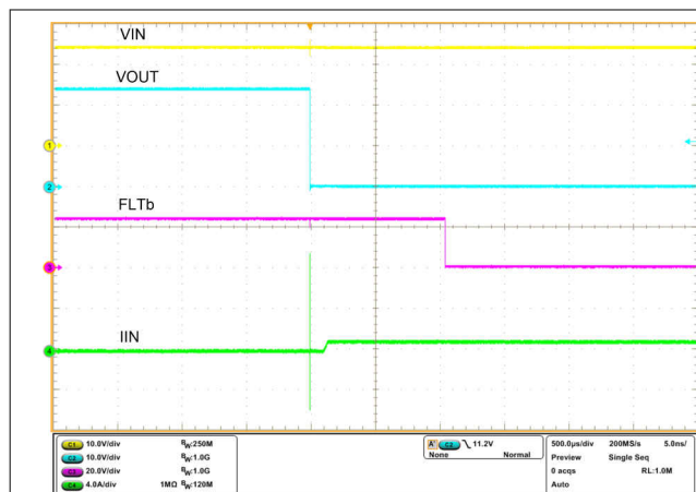
Figure 9-10. Output Hot Short Functionality at 24-V Input
