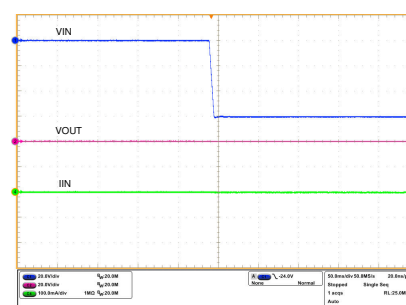
Reverse Input Polarity Protection at –60-V Supply
