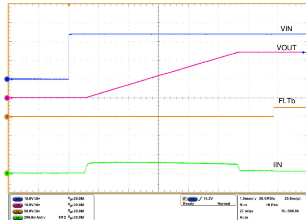
Figure 10-7. Hot Plug With VIN – No Load
