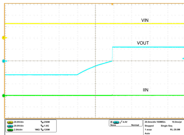
Figure 9-7. Response During Coming Out of Output Reverse Polarity Fault Condition
