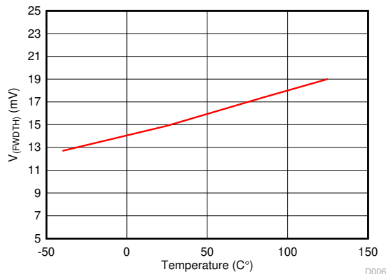
Figure 7-5. V_{F(WDTH)} vs Temperature
