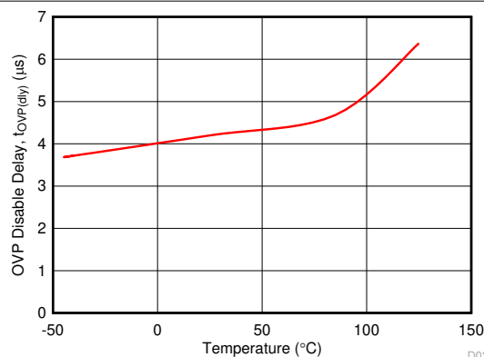
Figure 7-11. OVP Disable Delay vs Temperature
