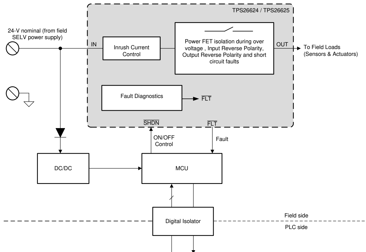
Figure 10-13. Power Delivery Circuit Block Diagram in I/O Modules
