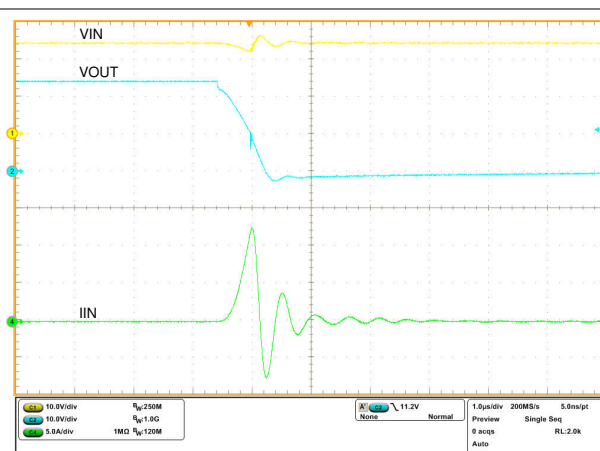
Figure 9-11. Hot-Short: Fast-Trip Response (Zoomed)
