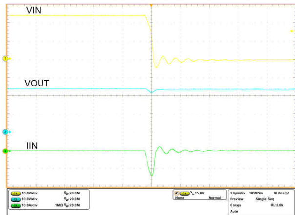
Figure 9-14. Hot-Short: Fast-Trip Response (Zoomed)
