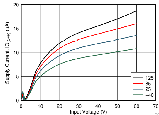
Figure 7-8. Input Supply Current vs Supply Voltage in Shutdown
