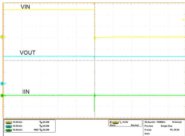
Figure 9-13. Input Hot Short Functionality at 24-V Supply
