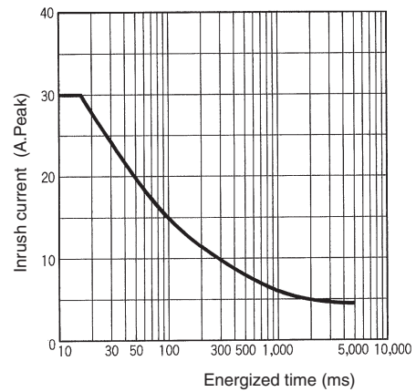
Inrush current resistivity
