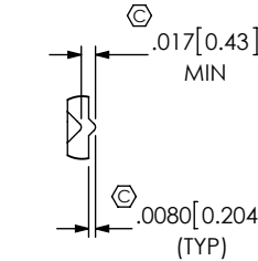
CRIMP DETAIL SCALE: 4:1 (TYP ALL CRIMPS)
