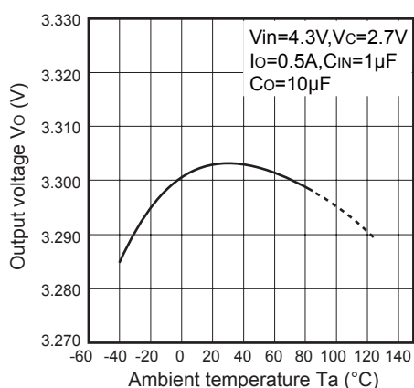
Fig.10 Output Voltage vs. Ambient Temperature (PQ033ENA1ZPH)
