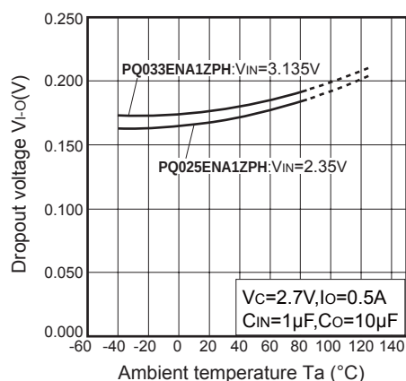
Fig.11 Dropout Voltage vs. Ambient Temperature (PQ025ENA1ZPH, PQ033ENA1ZPH)
