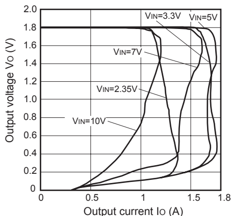
Fig.6 Overcurrent Protection Characteristics (PQ018ENA1ZPH)
