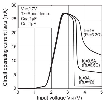
Fig.22 Circuit Operating Current vs. Input Voltage (PQ033ENA1ZPH)
