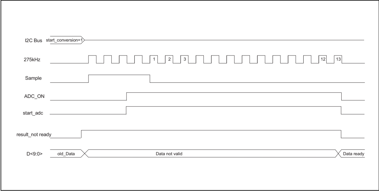
Figure 64: ADC Timing-diagram
