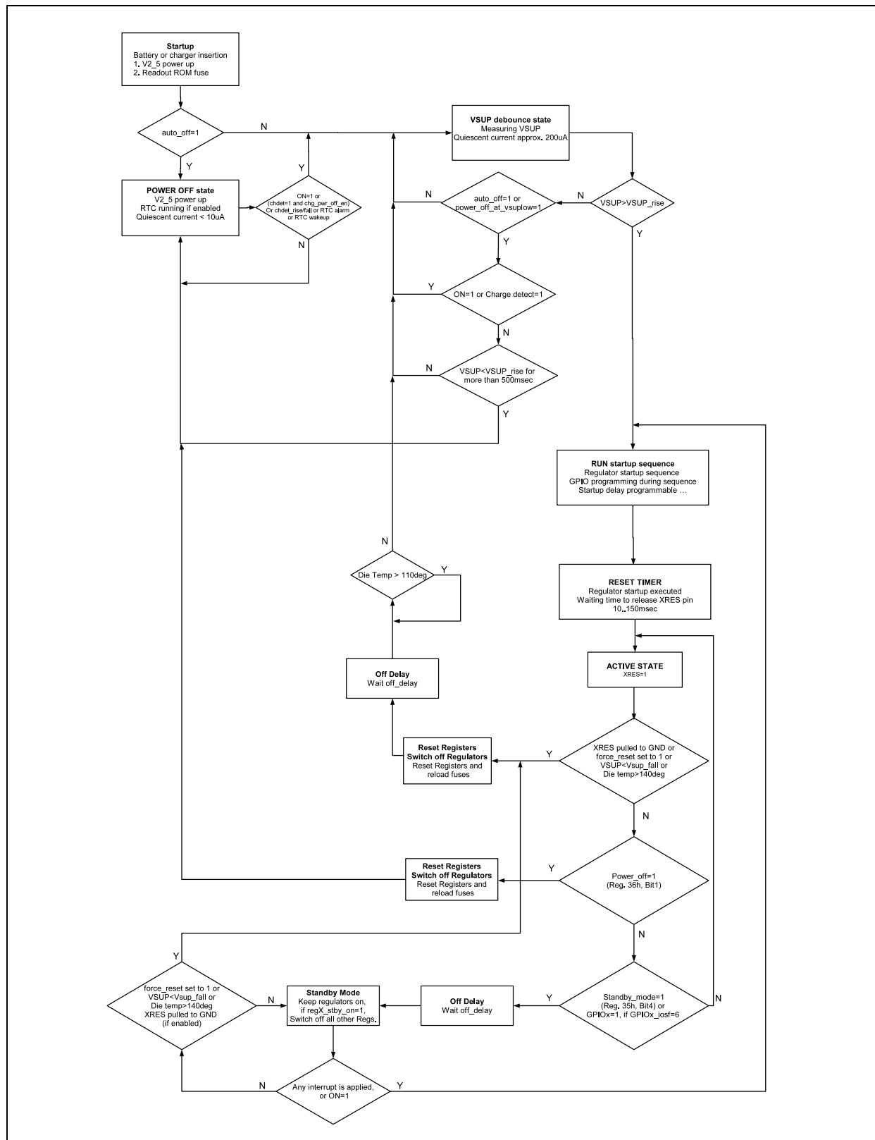
Figure 50: Startup Flow Chart
