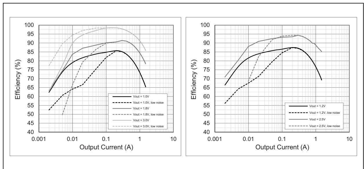
Figure 16: Step Down DC/DC SD1 Efficiency vs. Output Current; V_{SUP} = 3.0\text{V} , 3MHz operation, T_A = +25^\circ\text{C}
