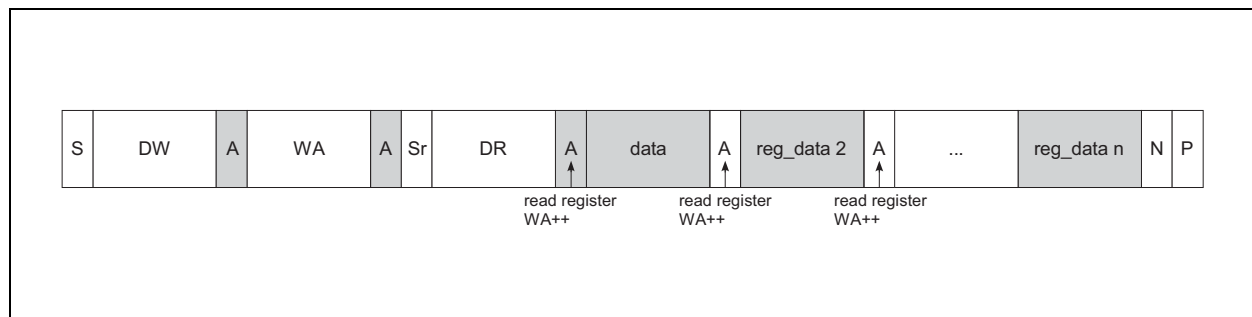
Figure 69: Sequential Read
