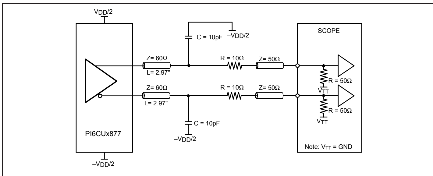
Figure 3. Output Load Test Circuit 2
