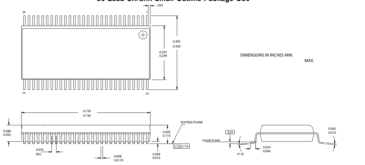
56-Lead Shrink Small Outline Package O56
