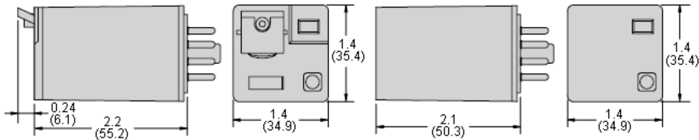
Plain Cover Dimensions
