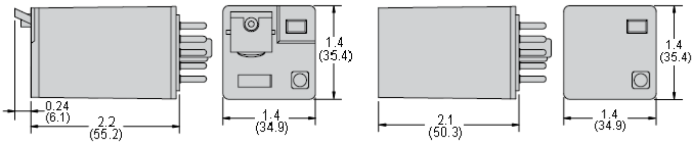
Full Featured Dimensions
