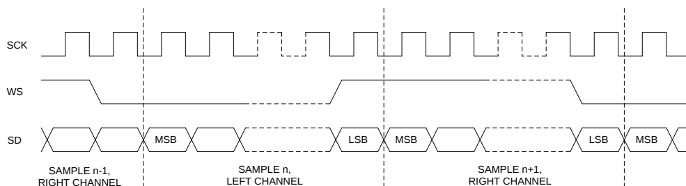
Figure 42: I 2 S Digital Audio Signaling
