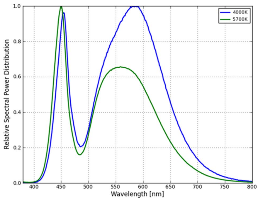
Figure 5. Color Spectrum of LIQ0-xx7000000zzz0.
