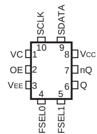
IDT8N3QV01 Rev G 10-lead Ceramic 5mm x 7mm x 1.55mm package body CD Package Top View
