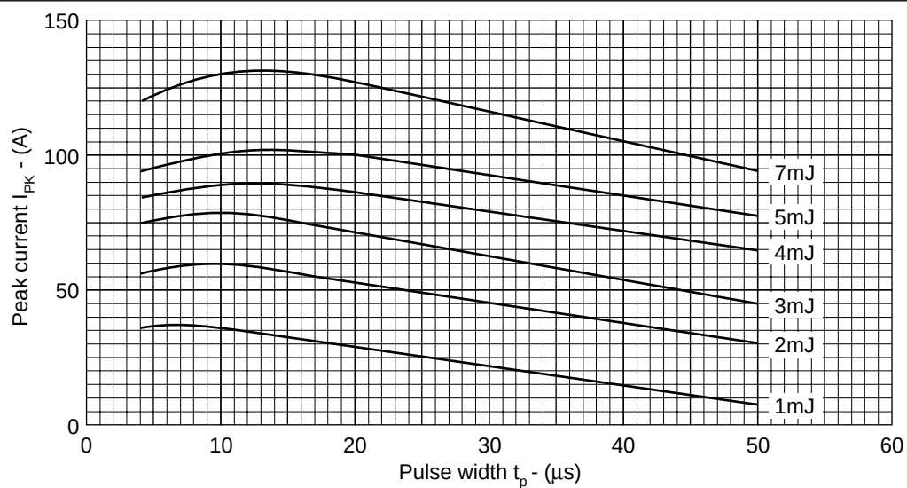
Fig.4 Maximum energy loss per pulse when switching a half sinusoidal pulse from 600V
