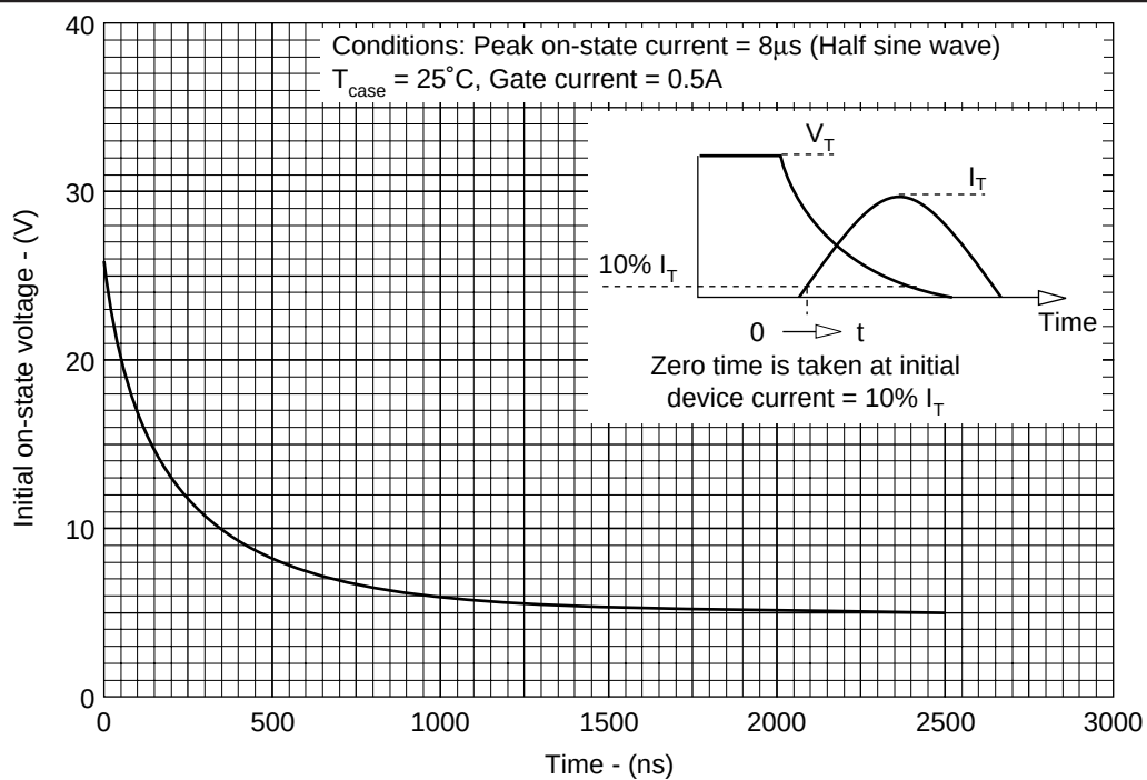
Fig.3 Typical initial on-state voltage vs time
