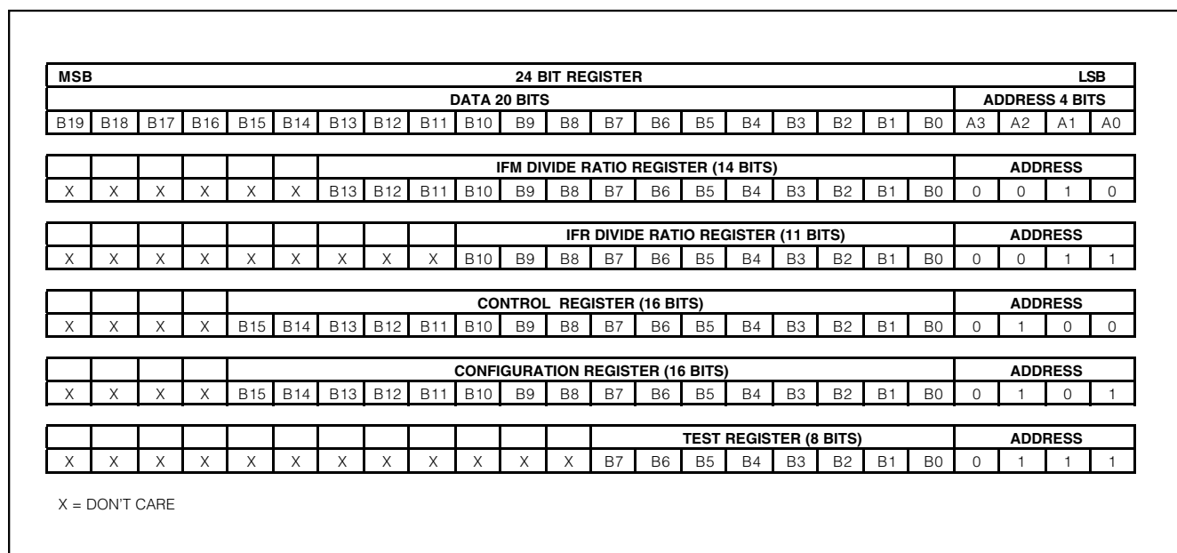
Figure 1. Register Configuration
