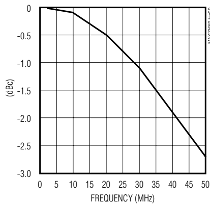
I/Q BASEBAND FREQUENCY RESPONSE
