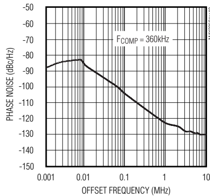
PHASE NOISE LOW-BAND OSCILLATOR vs. FREQUENCY OFFSET (181.26MHz)
