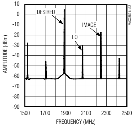
RFH OUTPUT SPECTRUM
