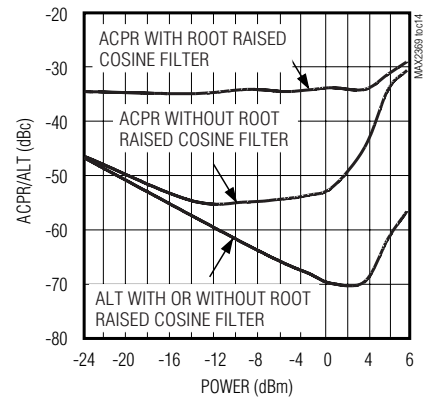
CASCADED ACPR/ALT vs. POWER (RFH)
