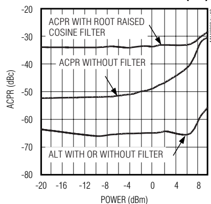
CASCADED ACPR/ALT vs. POWER (RFL)
