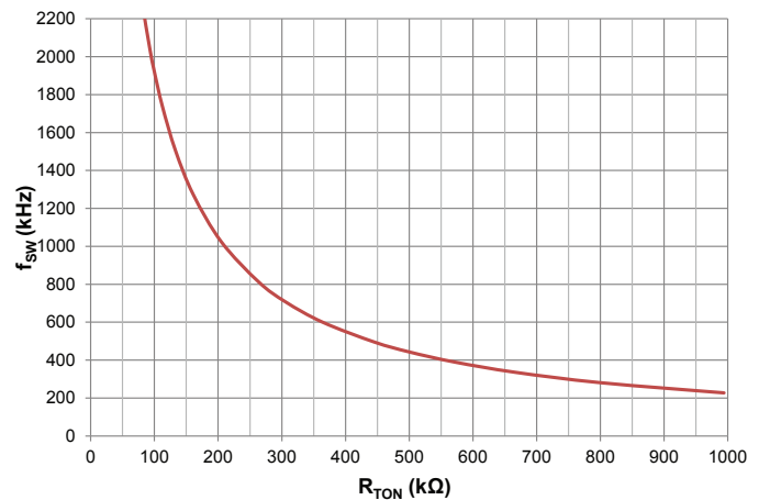
Figure 12: Switching Frequency vs. TON resistance
