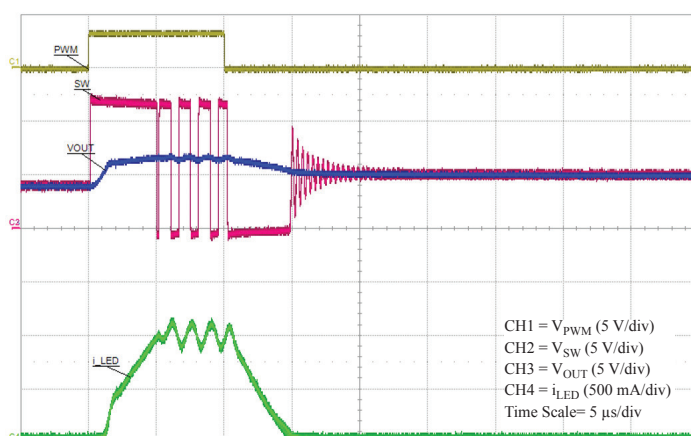
Figure 10: PWM Dimming with on-time of just 10 \mu s – R_{TON} = 442 \text{ k}\Omega , L = 22 \text{ }\mu\text{H} , V_{IN} = 12 \text{ V} , Output = 2 \times LED at 1 A. Note that the LED current takes \sim 5 \text{ }\mu\text{s} to ramp up to its steady-state value.
