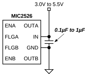
Figure 1. Supply Bypassing
