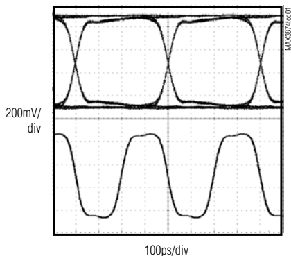
RECOVERED CLOCK JITTER (2.488Gbps)
