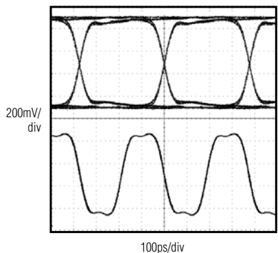
JITTER TOLERANCE (2.488Gbps, 223 - 1 PATTERN, V_{IN} = 10mV_{p-p} )
