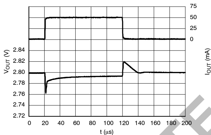
Figure 34. Load Transients, 2.8 V Version, I_{OUT} = 1 - 50 \text{ mA} , t_R = t_F = 0.5 \text{ } \mu\text{s} , V_{IN} = 3.8 \text{ V} , AE = V_{IN} \text{ V}
