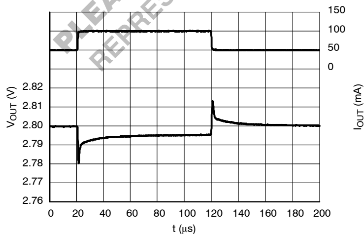
Figure 36. Load Transients, 2.8 V Version, I_{OUT} = 50 - 100 \text{ mA} , t_R = t_F = 0.5 \text{ } \mu\text{s} , V_{IN} = 3.8 \text{ V}
