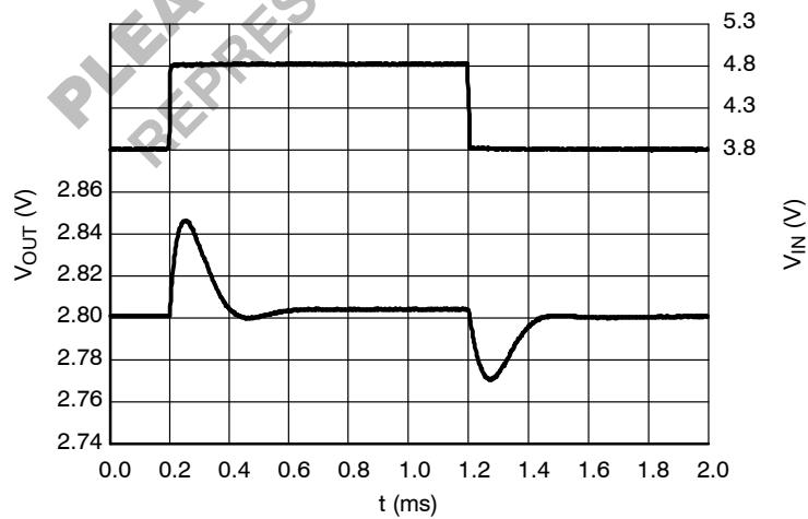
Figure 24. Line Transients, 2.8 V Version, t_R = t_F = 5 \text{ μs} , I_{OUT} = 1 \text{ mA} , AE = 0 \text{ V}
