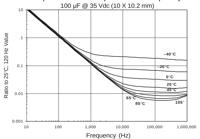
Impedance vs. Temperature & Frequency
