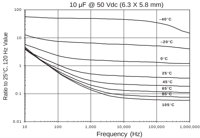
ESR vs. Temperature & Frequency
