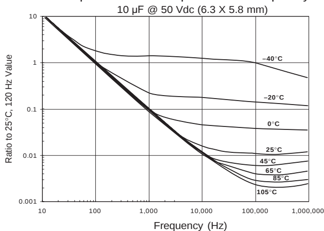
Impedance vs. Temperature & Frequency
