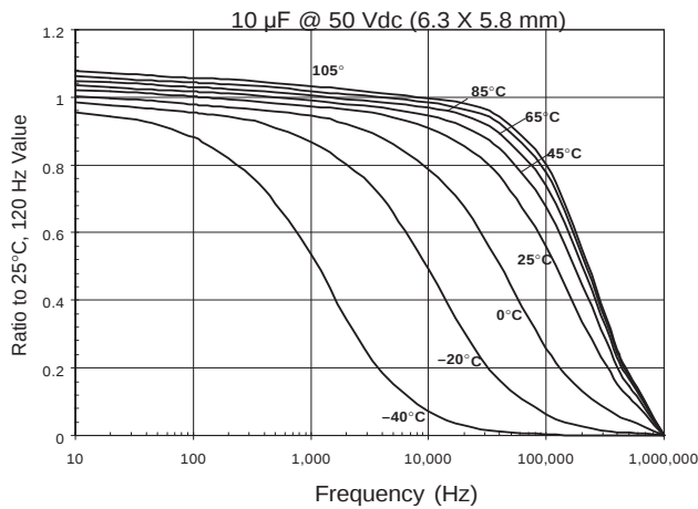
Capacitance vs. Temperature & Frequency
