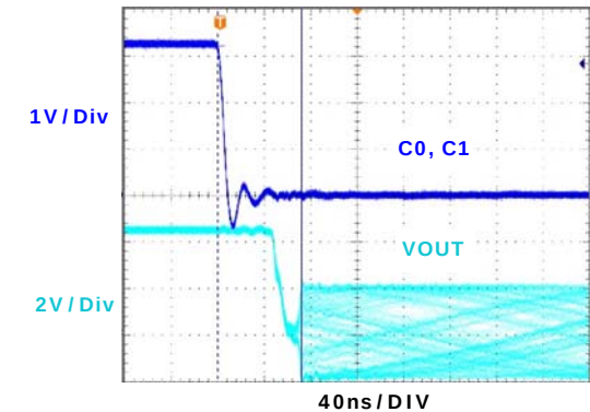
FIGURE 39. POWER-UP TIME
