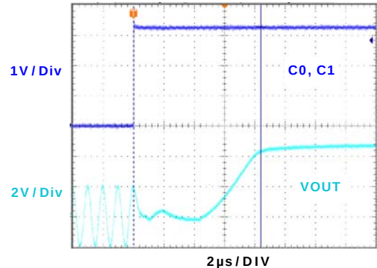
FIGURE 40. POWER-DOWN TIME
