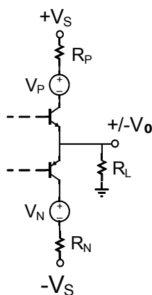
FIGURE 48. HEADROOM MODEL
