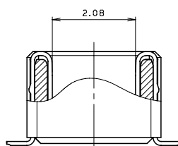
SECT. S-S
