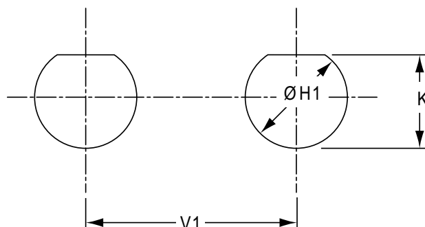
Jam Nut Receptacle (Type 24)
