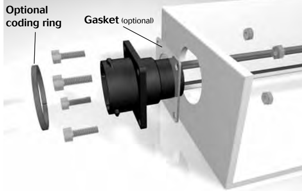
Front mounting : Solder version
