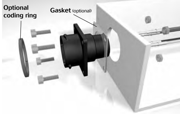
Front mounting : Crimp version
