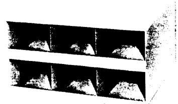
MODEL 921* Welding Rod Cabinet. Holds welding rod up to 18" long in six compartments. Each compartment is 18 \frac{3}{8} " deep x 4" high x 5 \frac{1}{4} " wide.
