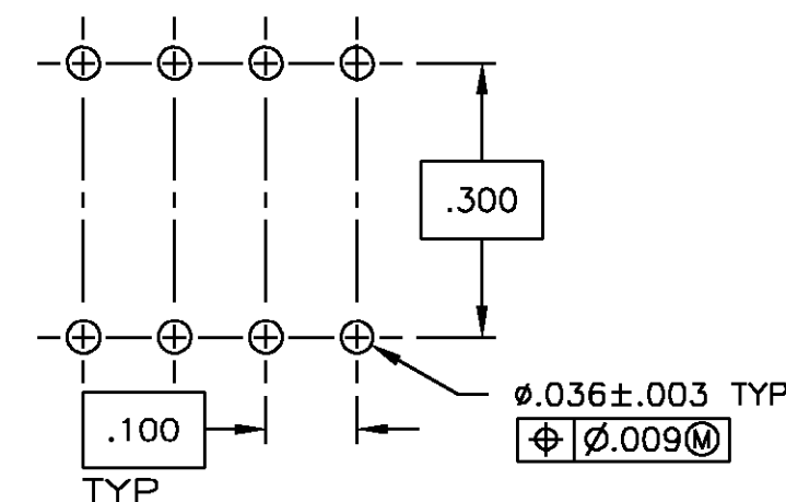
RECOMMENDED MOUNTING HOLE PATTERN SCALE 4:1
