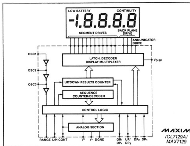
Figure 2. Simplified Block Diagram of MAX7129/ICL7129A Digital Section
