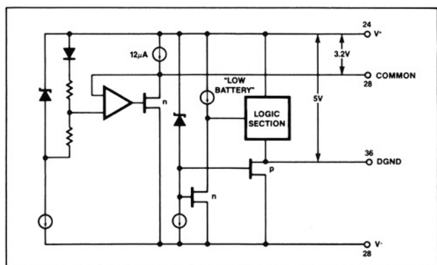
Figure 9. DGND and Common Outputs
