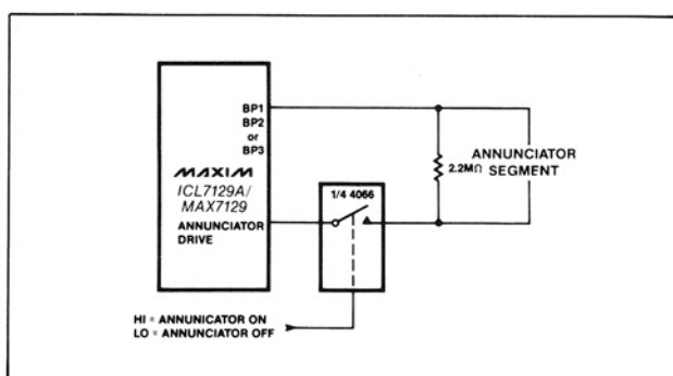
Figure 14. Externally Controlled Annunciators
