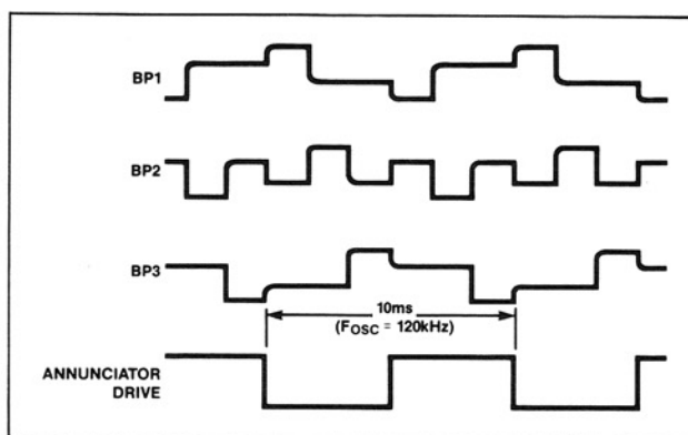
Figure 7. Backplane and Annunciator Drive Waveforms
