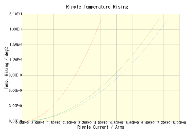
C3225X7R1E475K200AA(100kHz) C3225X7R1E475K200AA(500kHz) C3225X7R1E475K200AA(1MHz)
