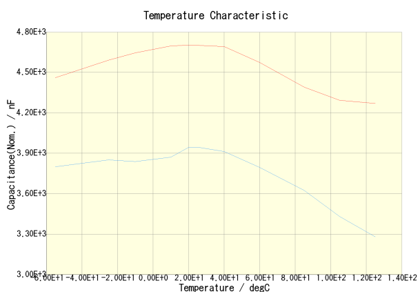
C3225X7R1E475K200AA(DC Bias = 0V) C3225X7R1E475K200AA(DC Bias = 12.5V)
